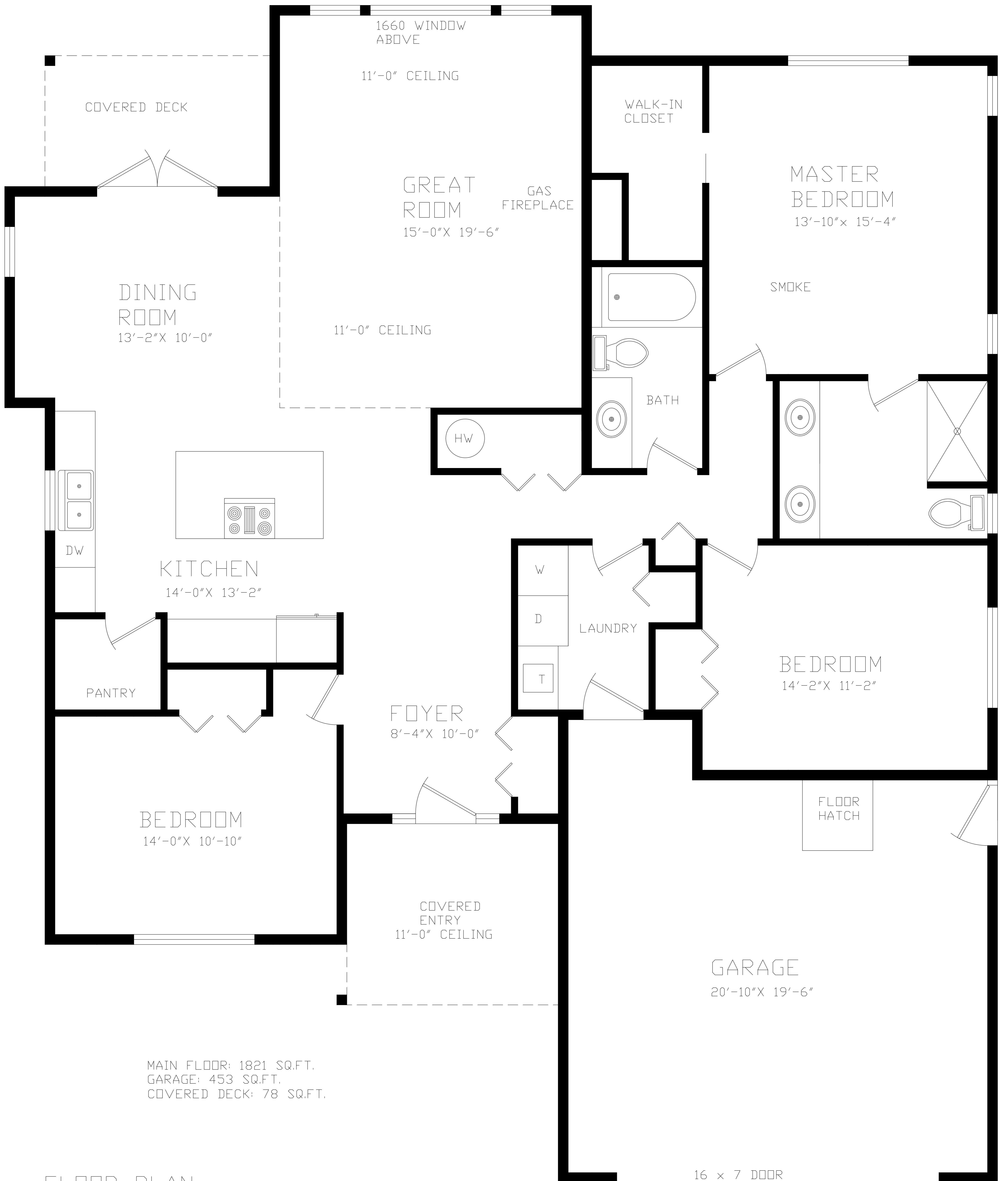
FLOOR PLAN
